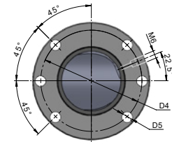
FLANGE TYPE 1
