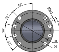
FLANGE TYPE 2
