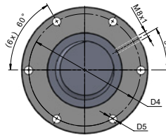
FLANGE TYPE 1
