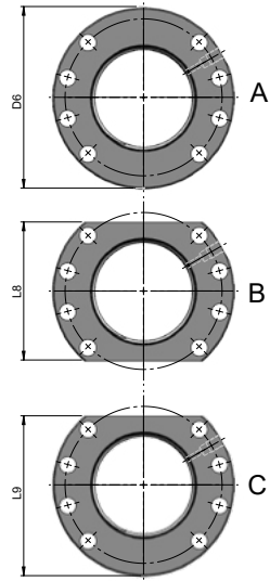
FLANGE FORM
