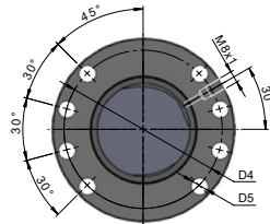
FLANGE TYPE 2
